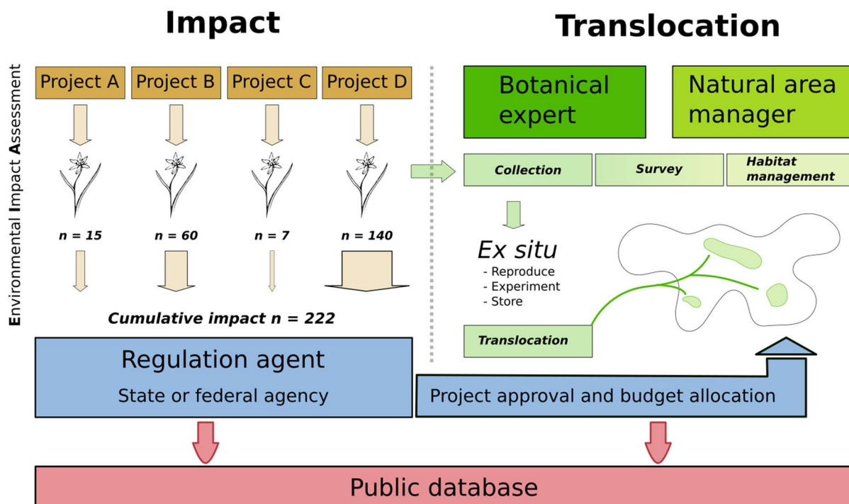
Fig. 4 Example of joint action of several stakeholders and development proponent/s to build a coherent translocation plan, with pooled funding, that will track cumulative impacts
