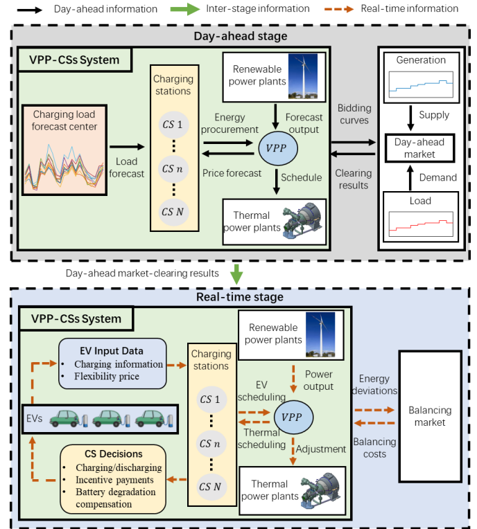
Fig. 2. Operation framework of the considered VPP-CSs system.
