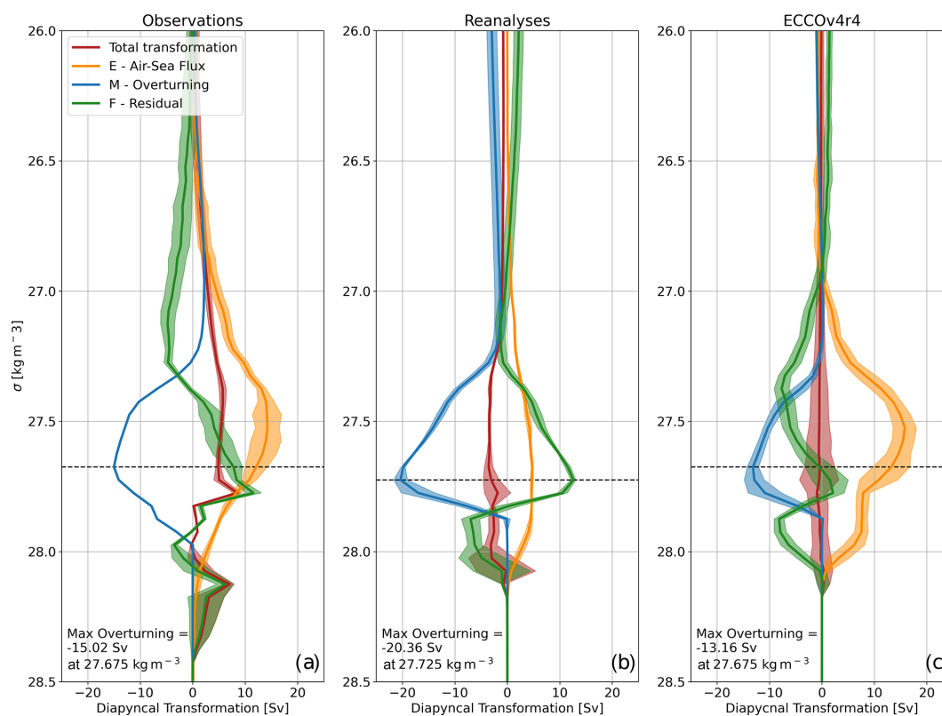
Figure 2. Time-mean diapycnal water mass transformation of the region to the north of the OSNAP section for (a) the observational dataset combination, (b) the reanalysis dataset combination and (c) ECCOV4r4. The panels show the volume tendency (red), the air–sea flux transformation (orange), the overturning streamfunction (blue) and the residual transformation (green). The shading in (a) and (b) represents the standard deviation of the respective dataset combinations. The shading in (c) represents the standard deviation of the annual means in ECCOV4r4.
