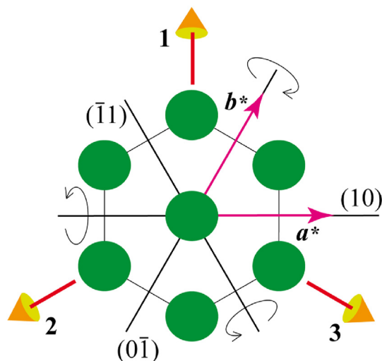
Fig. 6. View along the capillary axis of one of the four hexagonal domains. The columns point towards the reader and are represented by green circles. The reciprocal basis (a^*, b^*) is also represented. The other three hexagonal domains, whose axes are oriented along the directions 1, 2, and 3, are obtained from rotations of 109.5^\circ about the (10) , (11) and (0\bar{1}) reciprocal directions as shown.
