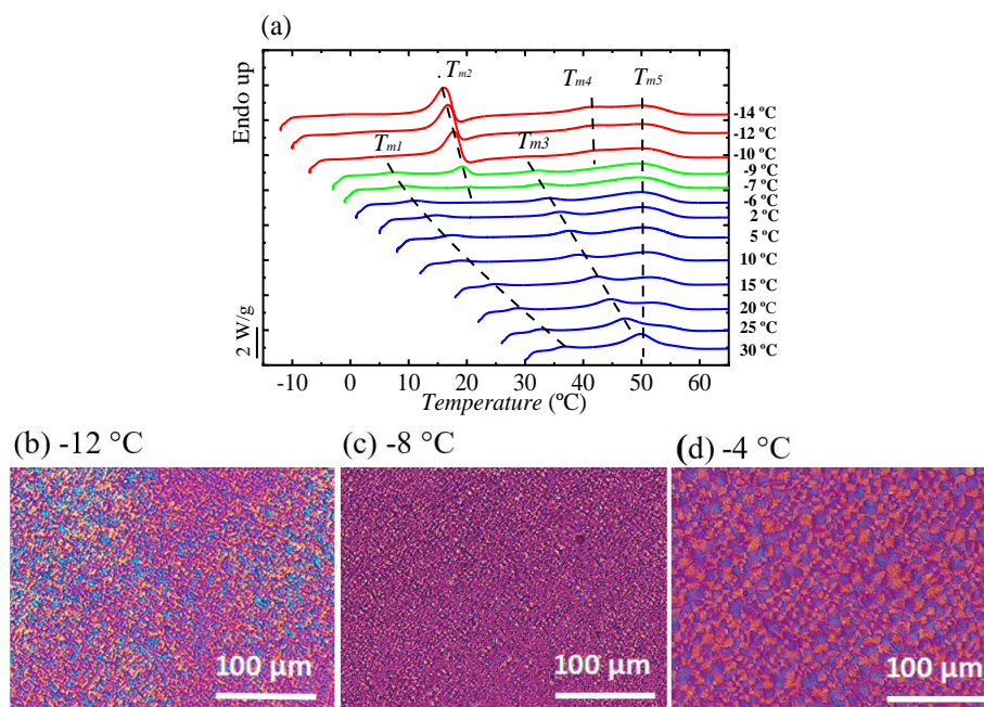
Figure 10. (a) DSC heating runs (at 10 °C/min) after isothermal crystallization at different temperatures. See text for the explanation of the color code employed. PLOM micrographs after isothermal crystallization at -12 °C (b), at -8 °C (c), and at -4 °C (d) for the BS 45 CL 55 sample.
