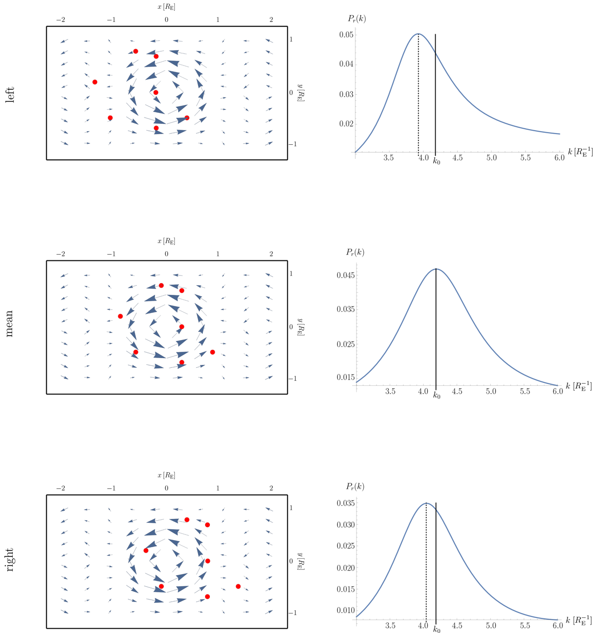
Figure 3. Reconstructed spectrum P_r(k) resulting from different measurement positions (red dots) with respect to the origin of the plasmoid. The length scale of the plasmoid is chosen to be k_0 \approx 4.19 R_E^{-1} .
