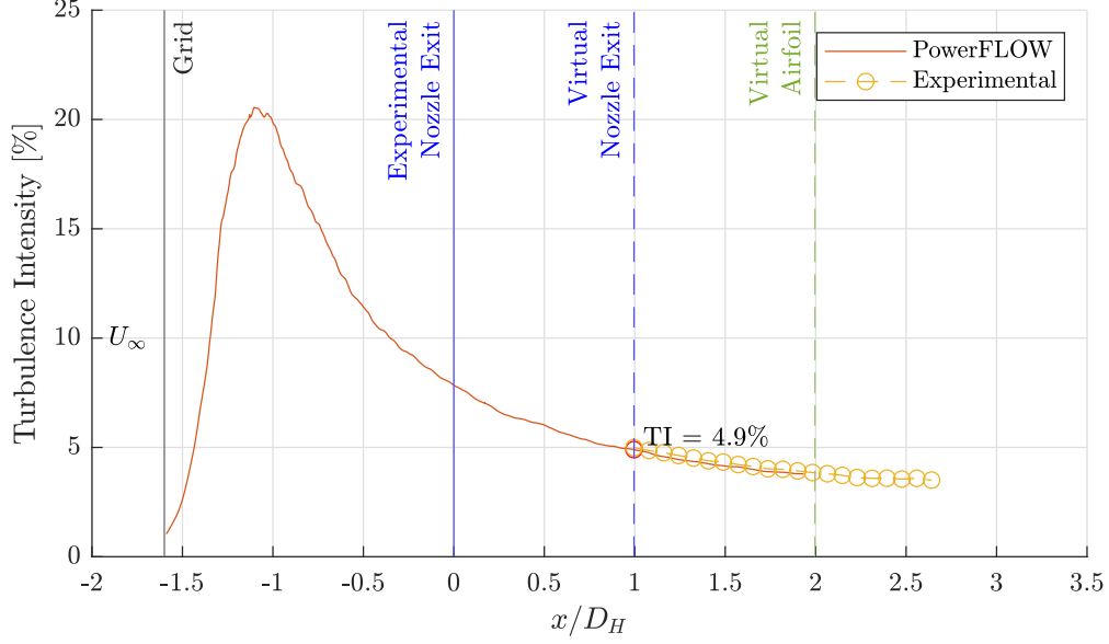
Fig. 4 Numerical and experimental results for turbulence intensity of the C2 grid.
