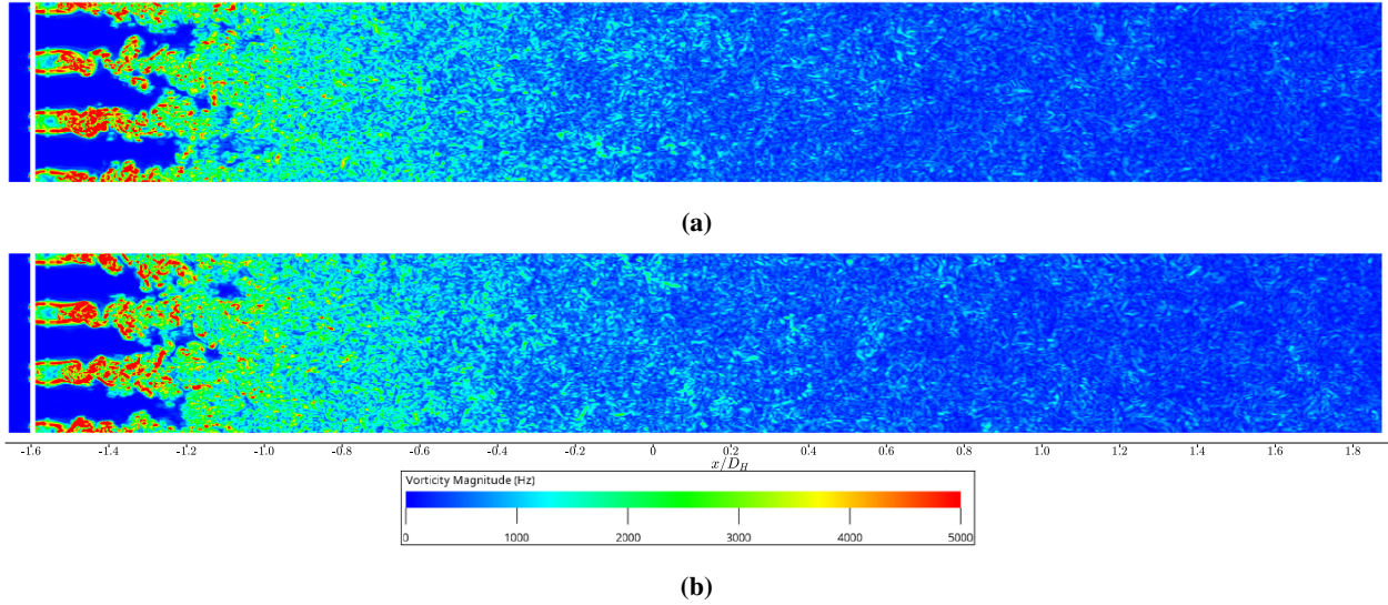
Fig. 7 Vorticity magnitude in the (a) span-wise ( y -aligned) plane and (b) cross-wise ( z -aligned) plane.
