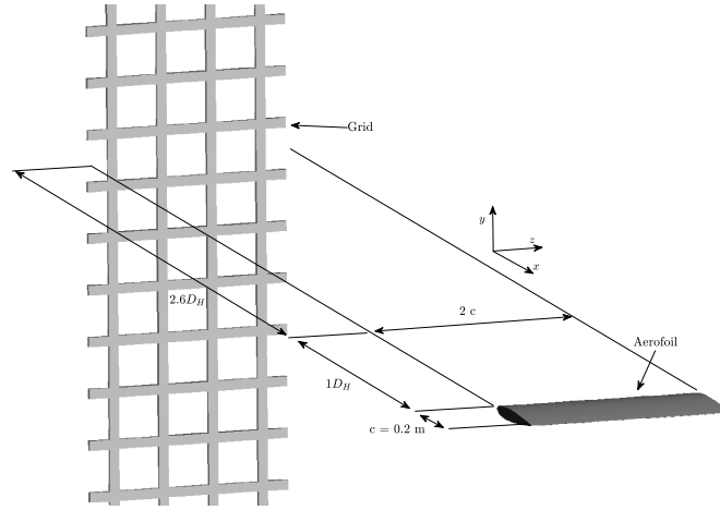
Fig. 6 Schematic of the grid-airfoil setup and coordinate system.
