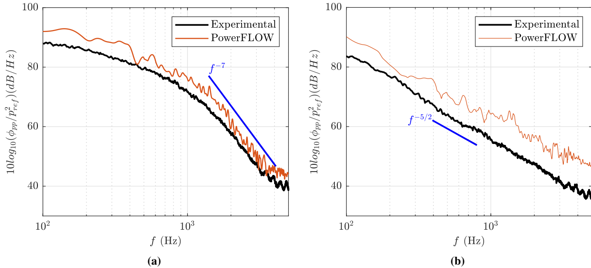
Fig. 10 Power Spectral Density of the surface pressure fluctuations comparison between experimental and numerical results over the NACA0012 airfoil for (a) transducer p1 located at the leading edge and (b) transducer p2 located at x/c = 0.08 .
