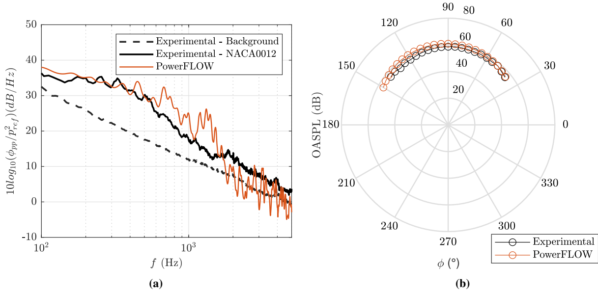
Fig. 9 Far field (a) Noise sound pressure level comparison between experimental data and solid FW-H from PowerFLOW simulation measured at \theta = 90^\circ and (b) Overall sound pressure level directivity comparison between experimental data and solid FW-H from PowerFLOW simulation
