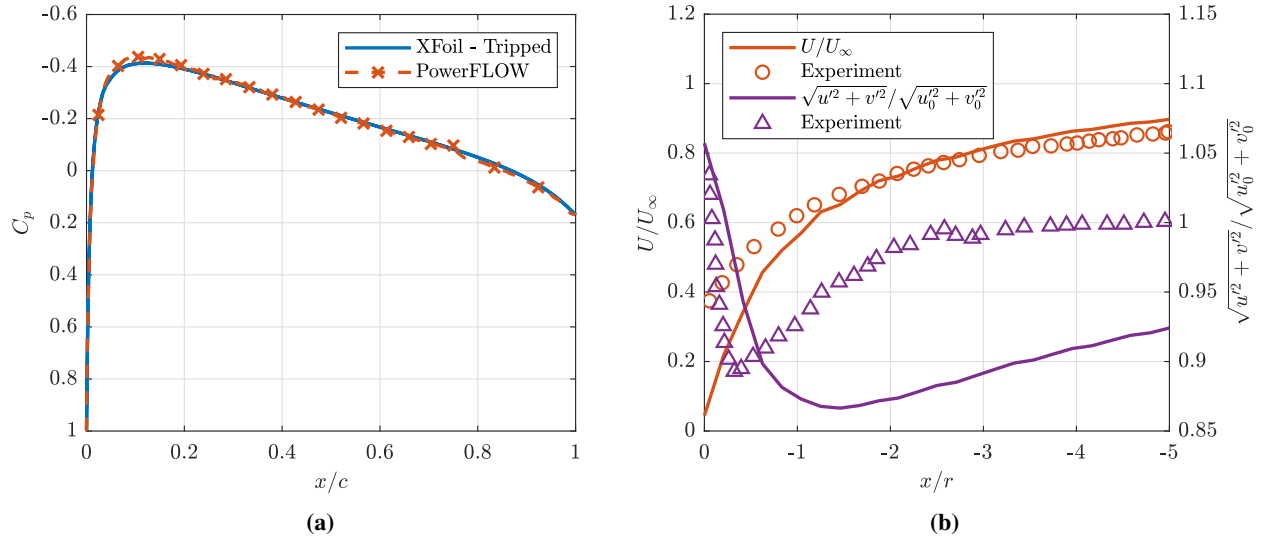
Fig. 8 Comparison of (a) Mean pressure coefficient C_p for the NACA0012 airfoil from XFOil and PowerFLOW and (b) Stagnation line evolution of the stream-wise component of velocity U/U_\infty (left axis) and root-mean-square of the velocity fluctuations \sqrt{u'^2 + v'^2} / \sqrt{u_0'^2 + v_0'^2} (right axis) from PowerFLOW (solid lines) and experiment (markers)
