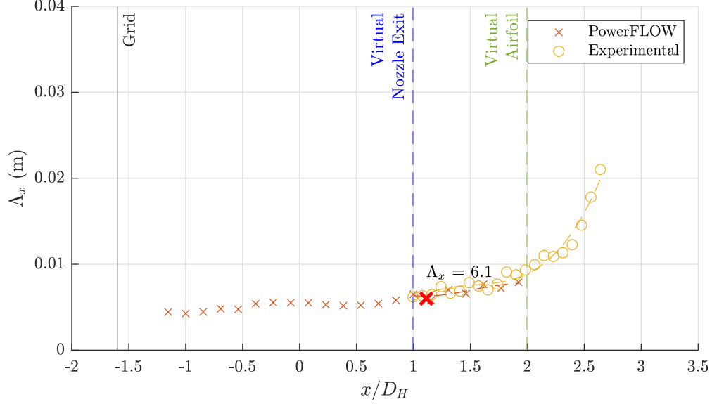
Fig. 5 Numerical and experimental results for integral length scale of the C2 grid.
