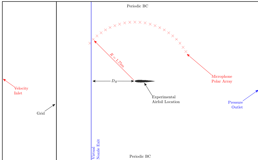
Fig. 3 Simulation setup for grid-generated turbulence, including the locations of the experimental nozzle exit and airfoil (boundaries and airfoil not to scale).
