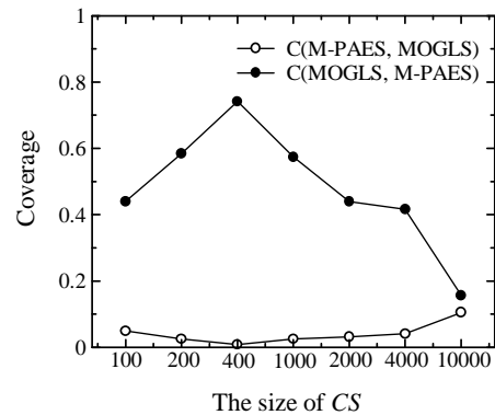
Figure 8: Results on the 2-500 problem. Different greedy repair algorithms were used in the MOGLS and the M-PAES.
