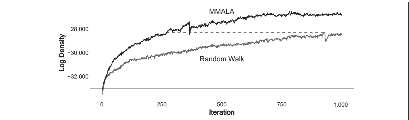
Figure 3. Illustration of IJC's faster rate of convergence with MMALA proposal distributions.
