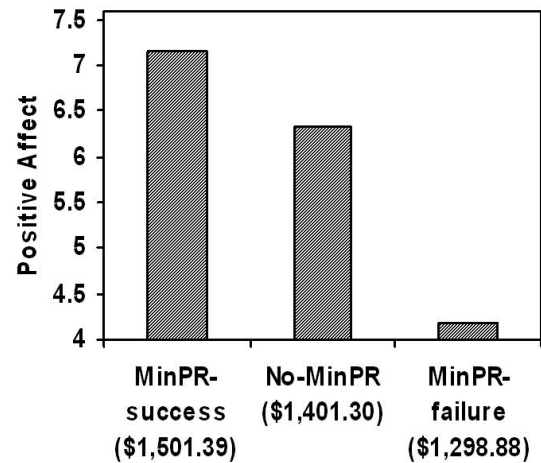
Figure 3. MinPR Effect
