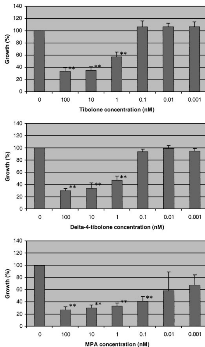
FIG. 3. Dose-response curve for PRAB-36 cells cultured in the presence of tibolone, \Delta^4 -tibolone, or MPA. Cells were cultured in the presence of different concentrations of tibolone ( top panel ), \Delta^4 -tibolone ( middle panel ), or MPA ( bottom panel ) for 10 d. Cells were harvested in 1 N NaOH, and OD 260 nm measurements were performed to measure cell growth. Cell growth is expressed as a percentage of control growth (Growth %). The experiments were performed three times, and paired-sample t tests were performed. Differences between control and treatments were considered significant (**) at P < 0.01. Each bar represents the average of three different experiments \pm SD.
