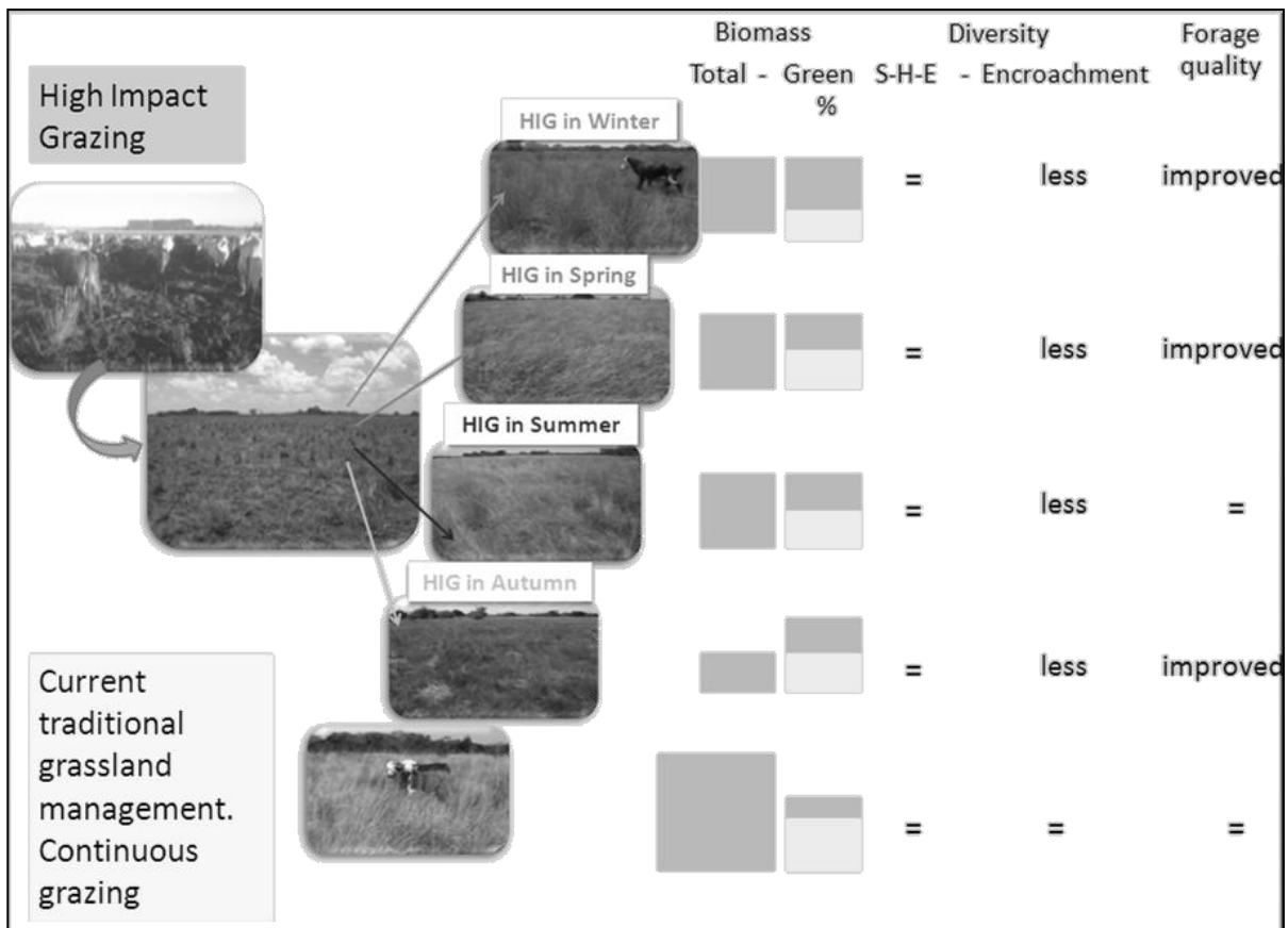
Fig. 5.1. Comprehensive diagram depicting the effects of high impact grazing (HIG) on biomass pools, species diversity and forage quality. (S = sp. richness; H = sp. diversity; E = sp. evenness).
