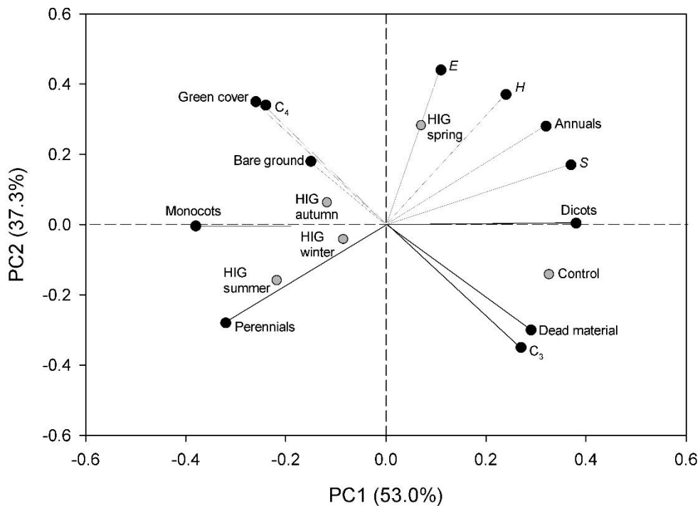
Fig. 3.2: Biplot of the PC1 (first principal component) and the PC2 (the second principal component), together they explain 90% of the data set variation (PC1 53% and PC2 37%). This figure represents the number of species, or species richness (S), species diversity (H) and species evenness (E). All other data expressed in %, green cover, dead material, annuals, perennials, C 3 (C 3 species cover), C 4 (C 4 species cover), dicots and monocots. High impact grazing (HIG) applied in winter, spring, summer or autumn.
