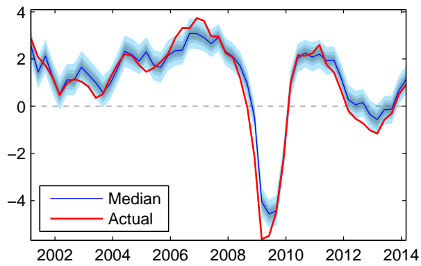
(a) Output approach: information set 1
