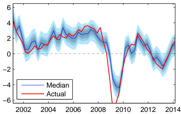
(a) Sectors G-H-I: information set 1
