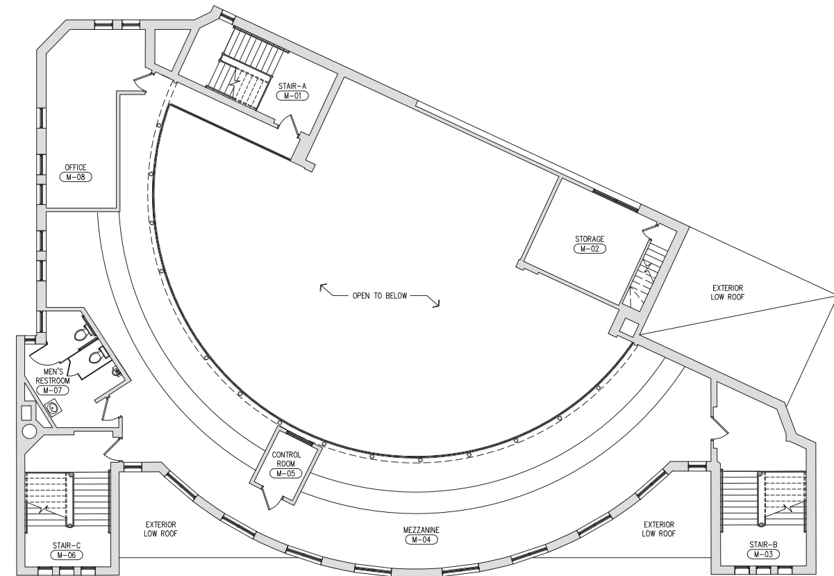
Mezzanine
