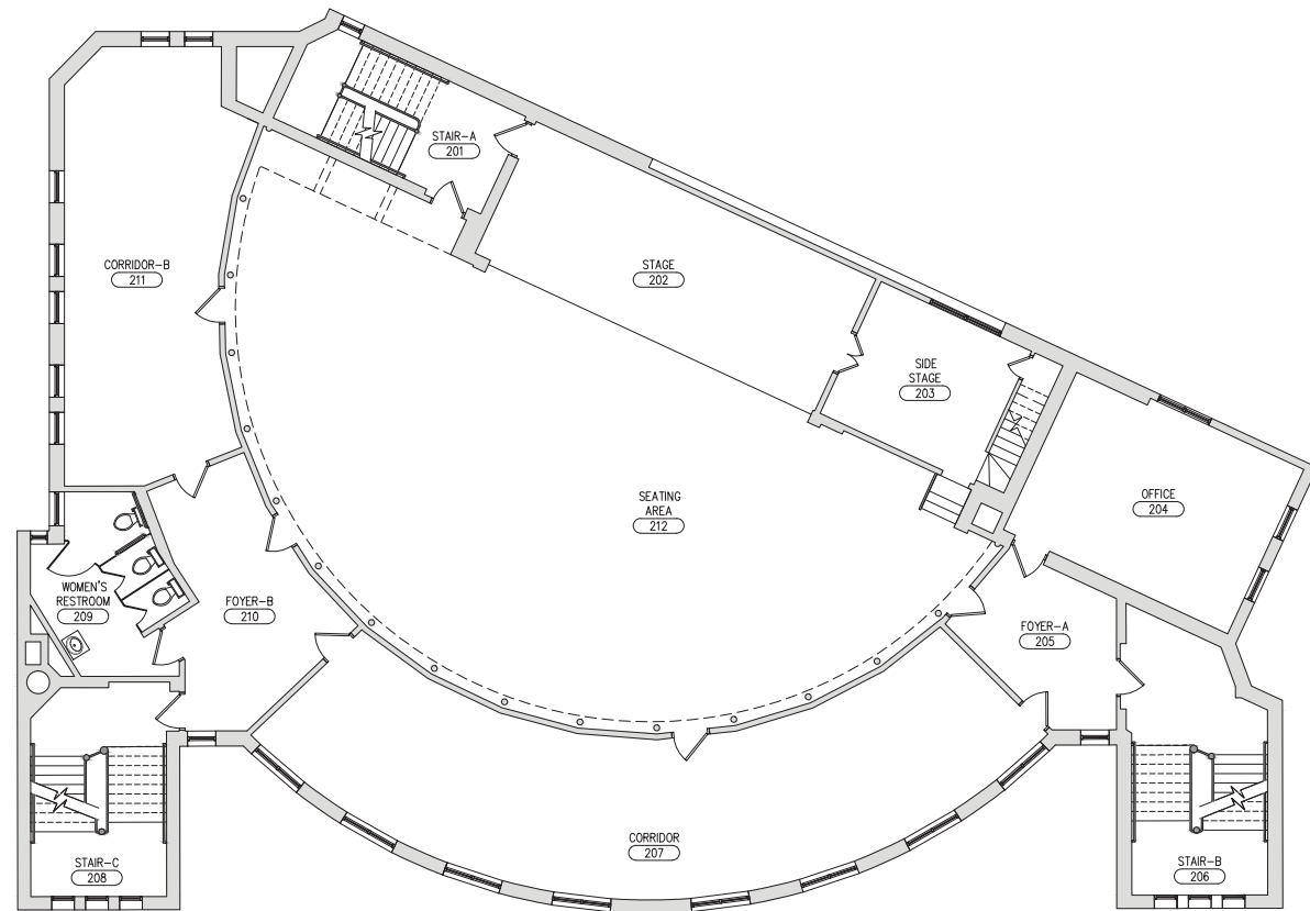
Second Floor
