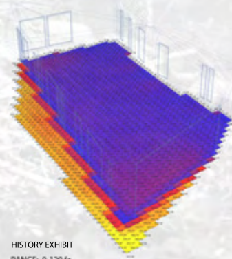
DAYLIGHT STUDY JANUARY 1, 2011 12:00 NOON
