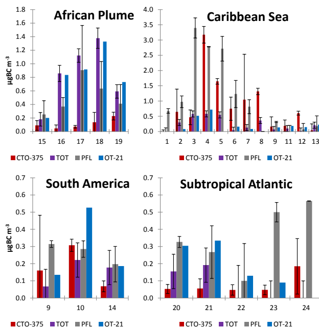
Figure 2. Comparison of black carbon concentrations ( \mu\text{g m}^{-3} ) from the four selected methods grouped by region with one standard deviation. Error associated with the OT21 method was \pm 0.1 \mu\text{g m}^{-3} .
