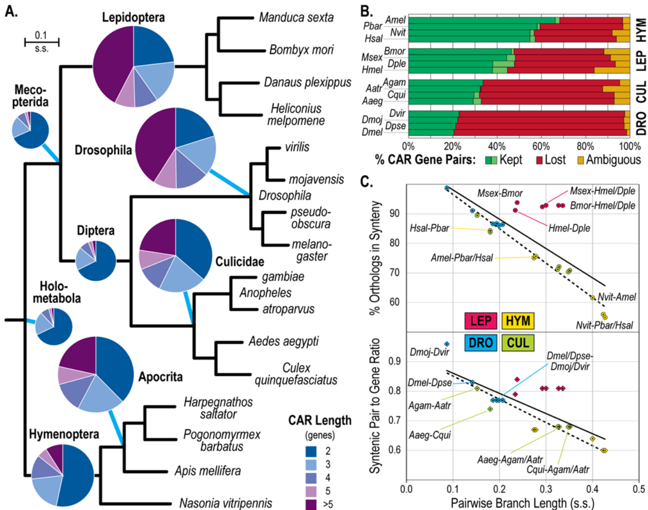
Figure 2. Remarkably conserved synteny among the Lepidoptera.
