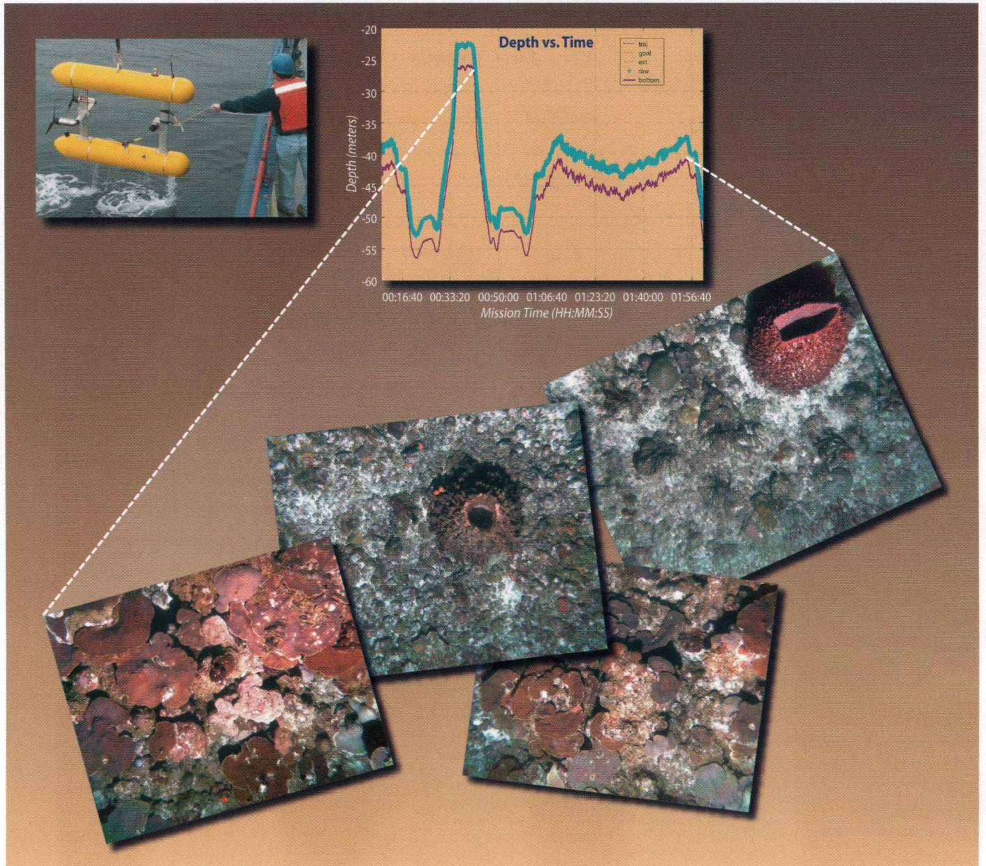
Fig. 1. The Seabed AUV (top left) has been designed for high-resolution imaging close to the sea floor. It is capable of working very close to the sea floor, as illustrated by the mission depth profile (top center) at a coral reef in the U.S. Virgin Islands. During this mission, it followed the sea floor bathymetry at a height of 3 m across a steep cliff in varied terrain. Even in such challenging environs, the Seabed AUV can obtain high-resolution, high-quality color imagery (bottom row).
