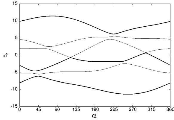
FIG. 11. Energy eigenvalues E_k , k=1, \dots, 6 in the invariant subspace of H_{A1A}^4 plotted vs \alpha on the path with radius \sqrt{A^2 + J_z^2} = \sqrt{0.3712} at J_y=0.4 off the integrability hyperboloid in (J_y, J_z, A) space.
