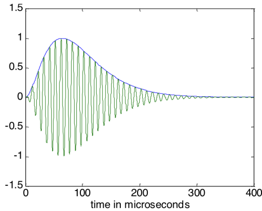
Figure 2: The Loran pulse, p(t) .
