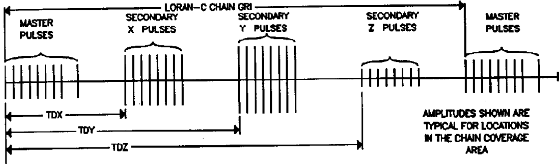
Figure 5: Entire chain timing, from [4].
