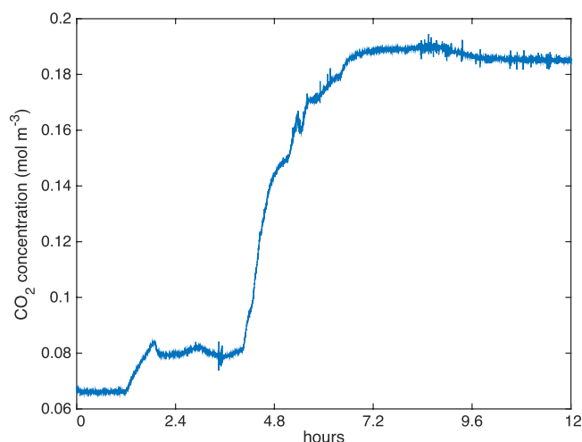
Figure 5. A time series of \text{CO}_2 addition to the test basin in preparation for a gas evasion experiment. The \text{pCO}_2 is measured every 2 s using a membrane contactor and Licor LI-840. As \text{CO}_2 -rich water from the 500 gal. tank is gradually added to the test basin, the water is rapidly mixed to produce a homogeneous concentration.
