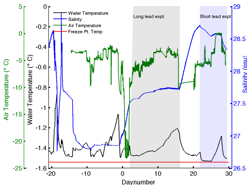
Figure 2. Air and water temperature as well as salinity of the test basin throughout the GAPS experiment. The red line indicates the freezing point temperature at 28.5 psu (−1.54°C). Daynumber = 0 corresponds to the day that the lead experiments began; the negative days numbering corresponds to the ice floe experiments not described in this manuscript.
