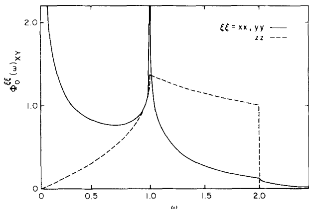
FIG. 2. Frequency-dependent autocorrelation functions \Phi_0^{xx}(\omega)_{XY} = \Phi_0^{yy}(\omega)_{XY} (solid line) and \Phi_0^{zz}(\omega)_{XY} (dashed line).
