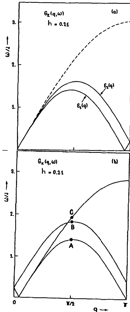
Fig. 7 Spin wave continua in a finite field in the thermodynamic limit, contributing to G_z (a) and G_x (b). For A, B, C see text. The dashed line in (a) indicates the h = 0 upper SWC boundary which becomes meaningless at finite h .
