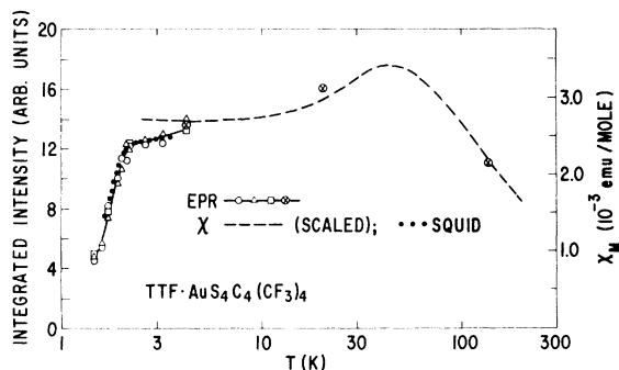
FIG. 7. Low-temperature powder magnetic susceptibility (SQUID magnetometer) and integrated EPR intensity with H along two major crystal axes for TTF \cdot AuS_4C_4(CF_3)_4 . These are scaled to match the static Faraday susceptibility results of Fig. 6 at 4 K. The resonance spectrometer sensitivity is calibrated for all data shown.
