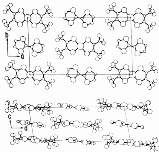
FIG. 4. View of the \text{TTF} \cdot \text{MS}_4\text{C}_4(\text{CF}_3)_4 , M = \text{Cu}, \text{Au} , structure in the a - b and a - c planes. \text{MS}_4\text{C}_4(\text{CF}_3)_4 anion is at the corners and face centers. The TTF cation is at the midpoint of each edge.
