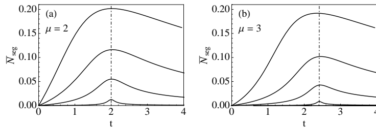
Figure 8. Density of segments, \bar{N}_{\text{seg}} , versus t at \tau = 1, 0.25, 0.05, 0.0025 (from top down) for (a) \mu = 2 and (b) \mu = 3 . The dot-dashed line marks t_0 .
