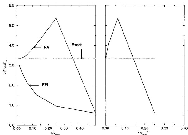
FIG. 1. The left panel compares the total energy of the double-well potential as a function of 1/k_{\max} determined using the virial estimator. The line labeled FPI represents the primitive Fourier method and the line labeled PA represents the results with partial averaging. The linear approach of the primitive Fourier results to the exact energy is characteristic of 1/k_{\max} convergence, and the approach with zero slope of the partial averaged results to the exact energy is characteristic of convergence that is more rapid than 1/k_{\max} . In the right panel the partial averaged results are plotted as a function of 1/k_{\max}^2 , and the linear behavior provides numerical verification of the asymptotic 1/k_{\max}^2 convergence rates of the partial average method. The error bars displayed in this and subsequent figures represent one standard deviation of the mean.
