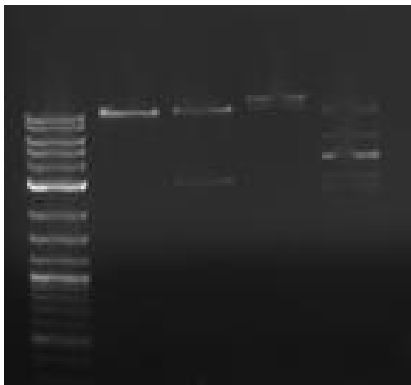
Figure 4: LR reaction of TD-miniSOG-P15r and miniSOG-P15r, using xt-18 as the destination vector. The bands represent in lane 2 confirm the expected 10177 and 2915 bp bands.
