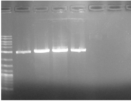
Figure 2: Restriction digest of plasmids from BP Reaction: Electrophoresis of the plasmid DNA isolated from the colonies that resulted from a BP recombination reaction cut with EcoRV.
