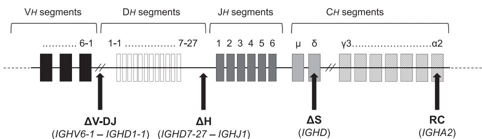
Fig. 1. Schematic depiction of the IGH@ gene complex (14q32.33). Arrows indicate the regions targeted by dPCR relative to the different genomic features of the gene complex. \Delta H is a mature B cell marker that becomes deleted due to the first VDJ rearrangement step (i.e. D-J joining) in the bone marrow during early B cell development. This marker is located between the IGHD7-27 and IGHJ1 genes. \Delta V-DJ is located between the IGHV6-1 and IGHD1-1 genes and is removed by a second subsequent VDJ rearrangement step (i.e. V-DJ joining). \Delta S is a switched B cell marker that becomes deleted by class switch recombination (CSR) in germinal centers during isotype switching of activated B cells. This marker is located in the constant gene IGHD . The regional corrector
