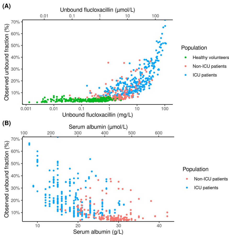
Fig. 1. Unbound flucloxacillin fraction versus unbound flucloxacillin concentrations (A) and versus serum albumin level (B).
