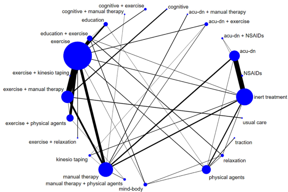
Figure 2. Network graph for pain at 1-month follow-up.
