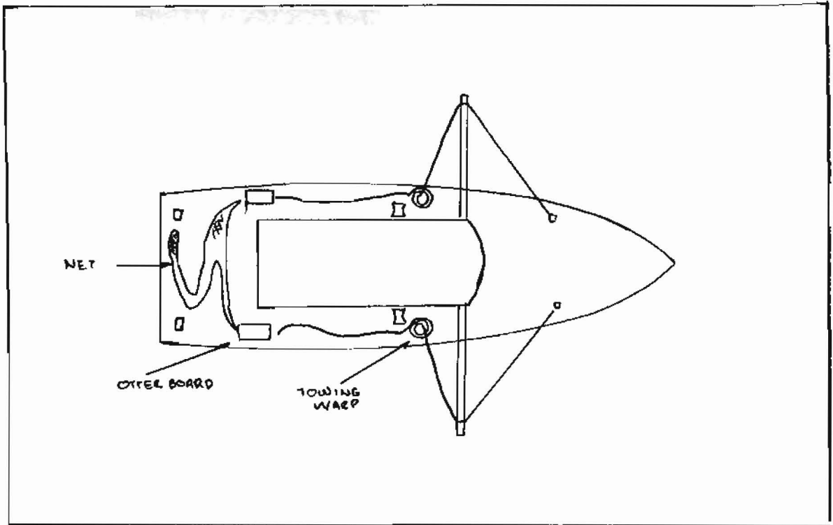
FIG. 3.0 DECK ARRANGEMENT OF TRAWLER READY FOR SHOOTING
