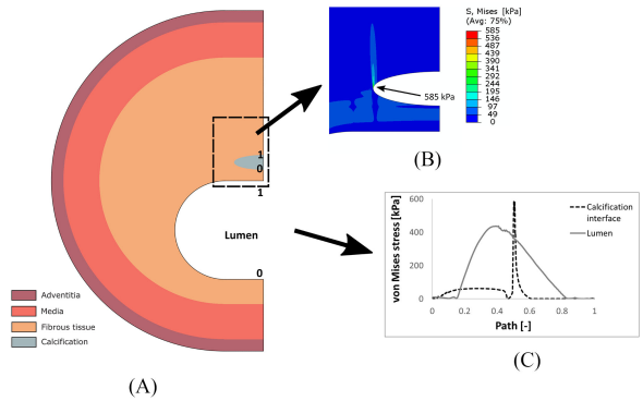
Fig. 5. (A) A representative finite element model of the attached fiber pattern with RL_{norm} = 0.15 , AR = 3.9 and W_{norm} = 0.12 , and (B) the corresponding von Mises stress distribution in the fibrous plaque tissue around the calcification. (C) the von Mises stress distribution along the calcification interface path and lumen path. The path start point (0) and end point (1) are indicated in the model (A) for both the lumen and the calcification interface. The maximum plaque tissue stress is 585 kPa and located at the calcification-tissue interface, whereas the highest stress at the lumen is 435 kPa.
