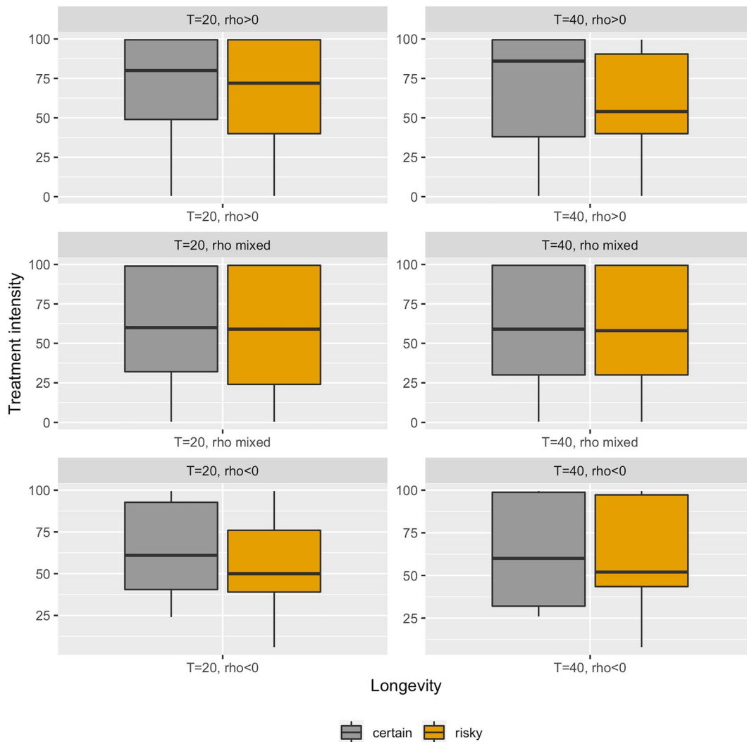
FIGURE 4 Relations between variation in treatment intensity and risk attitudes
