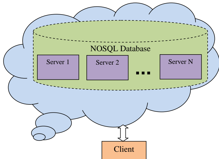
Figure 2.2 NoSQL Database
