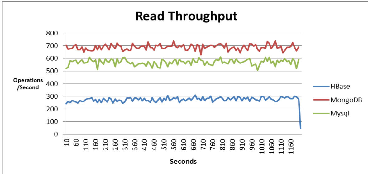
Figure 4.3 Read throughput
