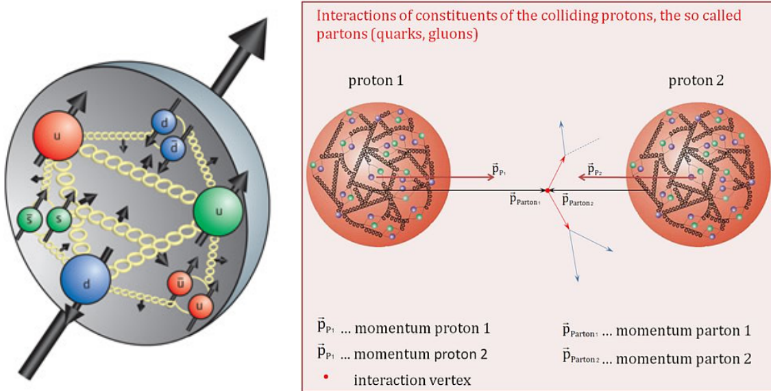
Figure 3.1: An illustration schematic diagram of the internal structure of a proton with two valance up quarks and one valance down quark which interact via gluons (left). The figure (right) shows a couple of protons about to collide where, a “sea” of quarks and gluons in addition to the valance quarks exist.[40]
