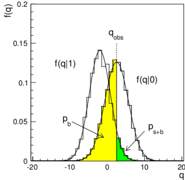
Figure 12.1: The distribution of the variable q of equation 12.1 under null and alternative hypothesis. [93]
