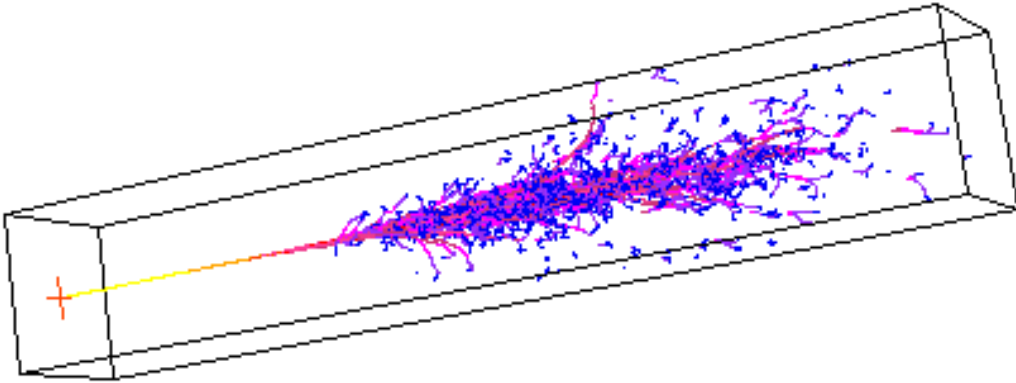
Figure 4.10: Simulation of showering of an electron in a PbWO 4 crystal of the CMS detector[70]
