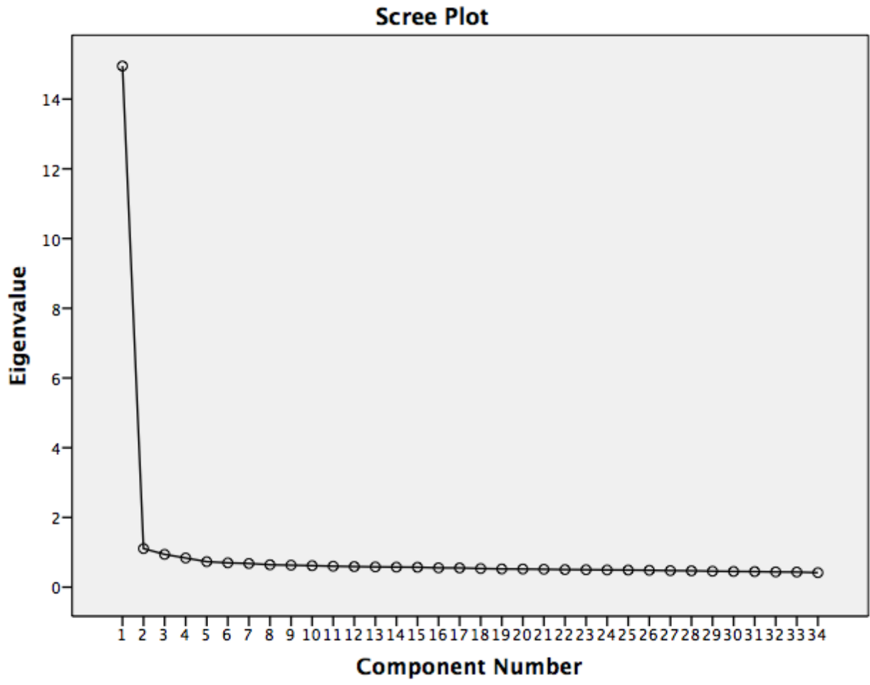
Figure 1. EFA screeplot
