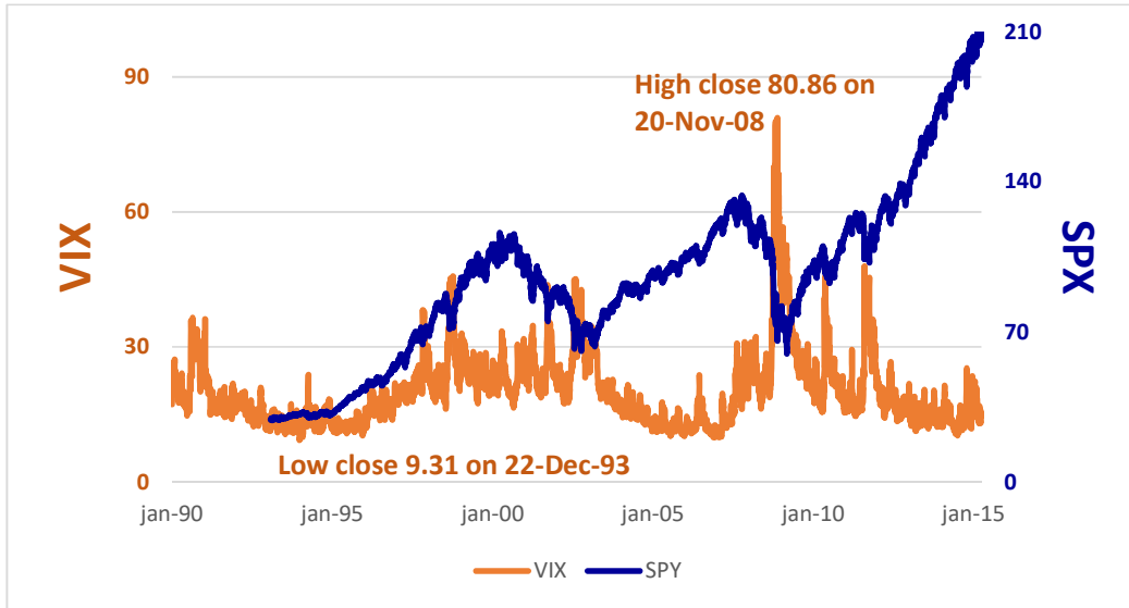
VIX and S&P 500 (SPX)
