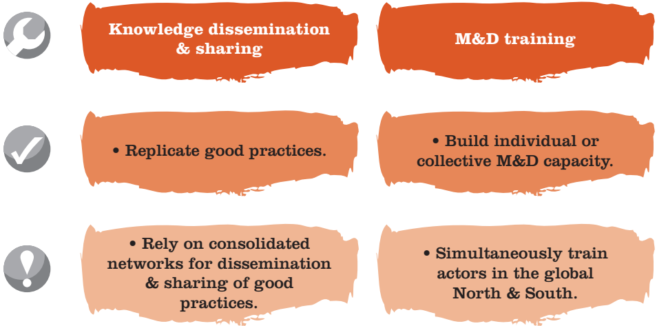
Figure 4: Network empowerment
