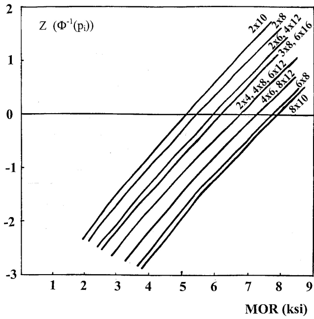
Figure 2. CDF of MOR for Douglas Fir Planks, Select Structural Grade
