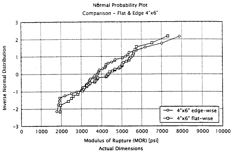
Figure 4. CDF of MOR for 4x6 Planks, Edge-wise vs Flat-wise Loading
