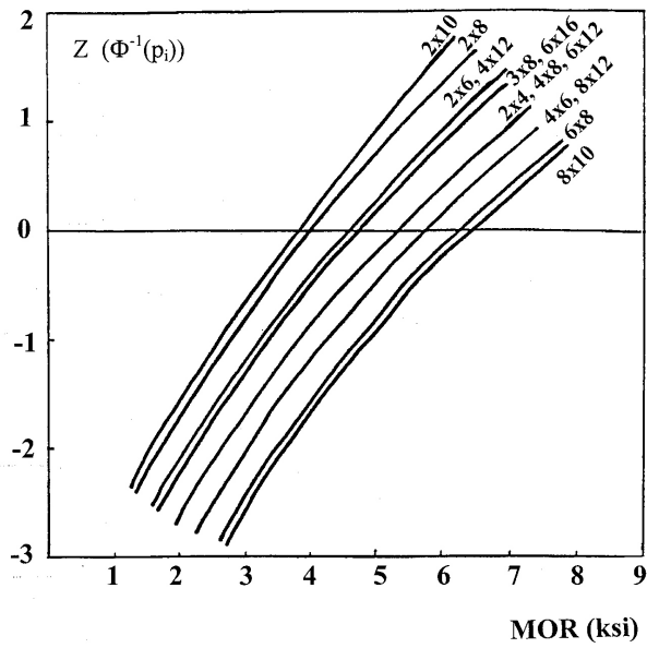
Figure 3. CDF of MOR for Douglas Fir Planks, Grades 1 and 2
