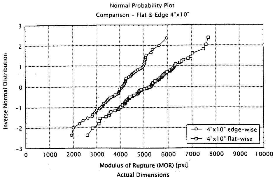
Figure 6. CDF of MOR for 4x10 Planks, Edge-wise vs Flat-wise Loading
