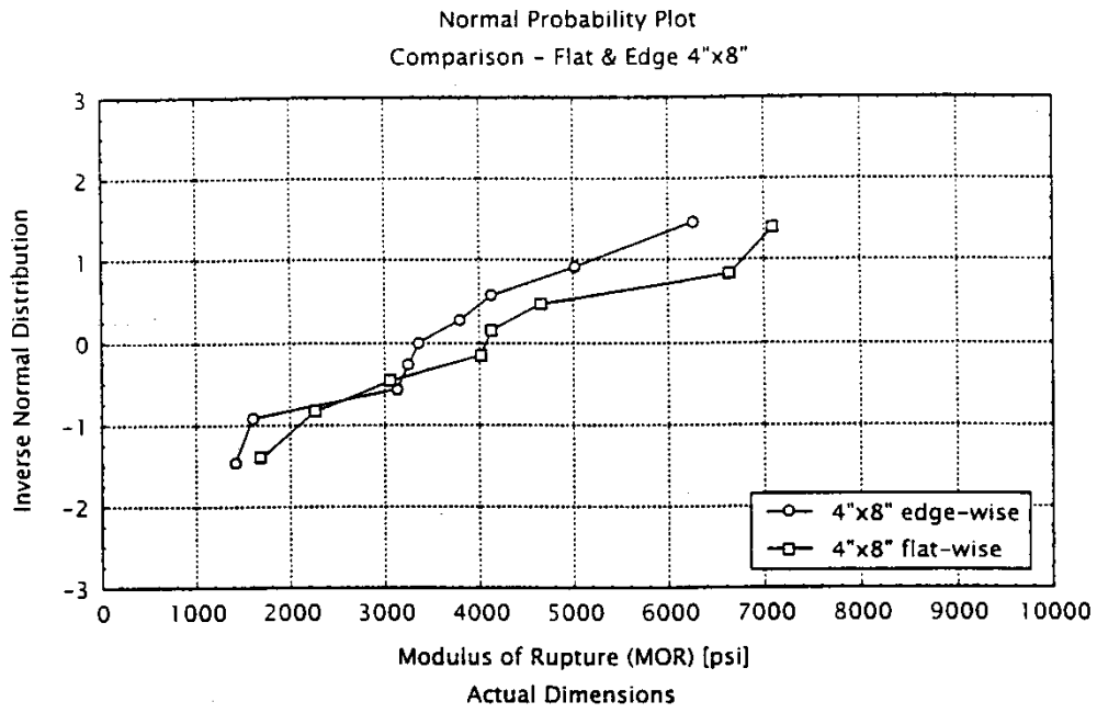
Figure 5. CDF of MOR for 4x8 Planks, Edge-wise vs Flat-wise Loading
