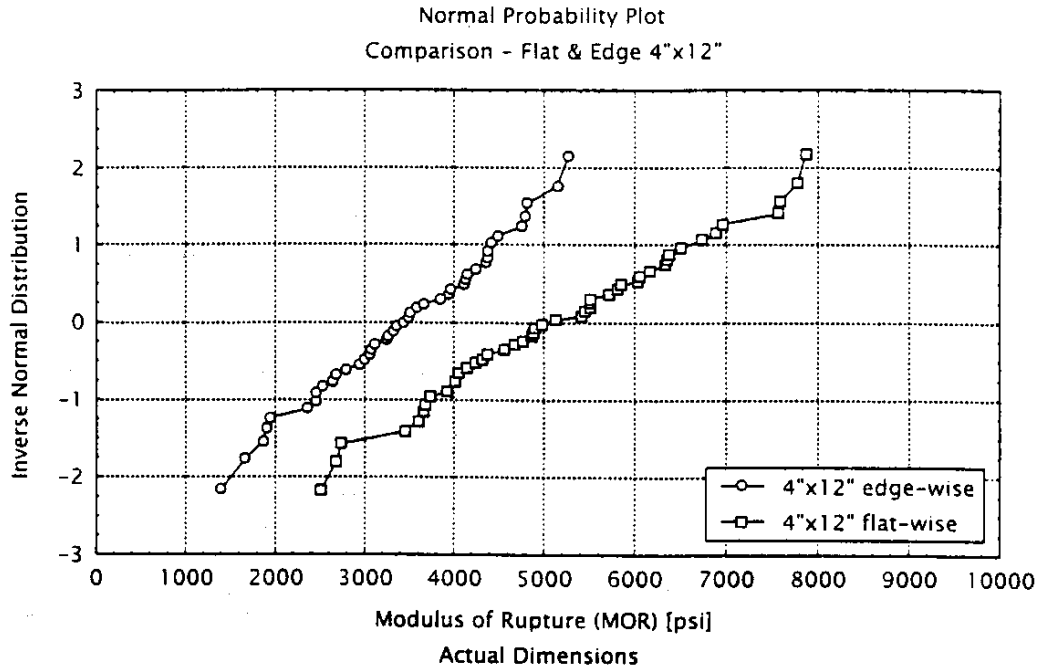
Figure 7. CDF of MOR for 4x12 Planks, Edge-wise vs Flat-wise Loading
