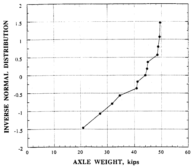
Fig 1. Cumulative Distribution Function of Maximum Axle Weight
