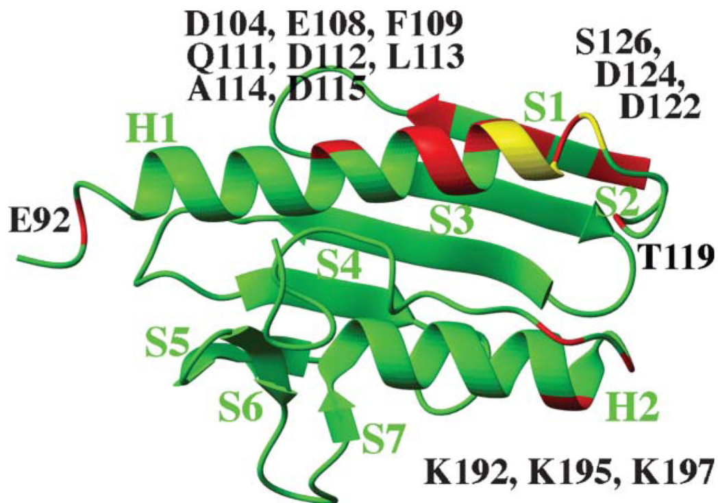
Fig. 2. Human frataxin residues perturbed at their amide position upon forming a complex with iron and ferrochelatase. Unshifted (green) and shifted (red) residues identified on the apo-protein's structure. Yellow residues are line broadened beyond recognition resulting from Fe binding.
