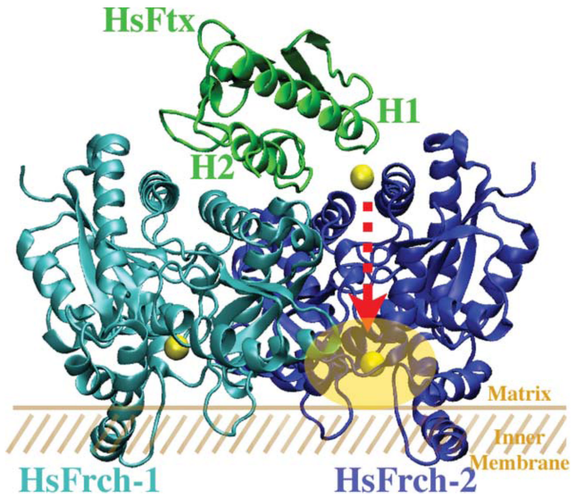
Fig. 3. Docking simulation of frataxin (Ftx) (green) with the ferrochelatase (Frch) dimer. Frataxin interacts with ferrochelatase on the matrix exposed side of the protein dimer during iron delivery (yellow ball). Delivered iron would then be available to be transported down ferrochelatase's substrate channel (red arrow) towards the enzyme's active site (yellow oval) located on the membrane side of the molecule.
