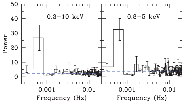
Figure 3. Average PDS extracted from the 0.3–10 keV (left) and 0.8–5 keV (right) light curves binned on 10 s, made from five segments of the light curve including the white noise (horizontal dashed line). There is an excess of variance at \sim 0.7 mHz which is significant at >3\sigma in the 0.8–5 keV band. As the power over the remaining observable frequency bins is consistent with the statistical white noise (possibly indicating the source as being stream-fed), this is an acceptable method for determining the significance of this feature.
