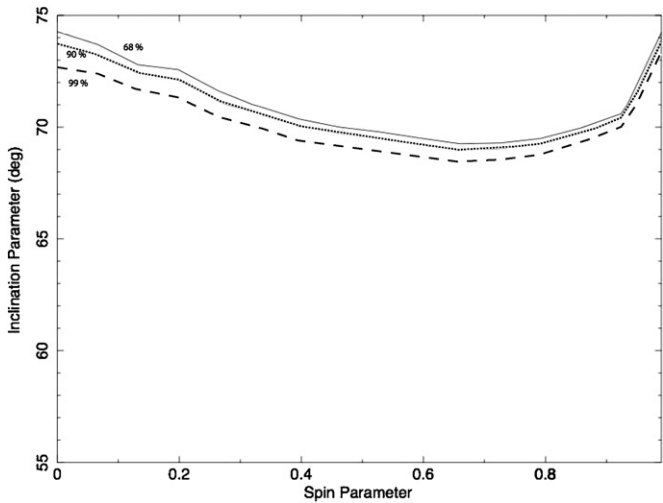
Figure 8. Inclination vs. spin contour plot for GRS 1915+105 using the reflionx model. The solid, dotted, and dashed lines show the 68%, 90%, and 99% confidence range for two parameters of interest, respectively.
