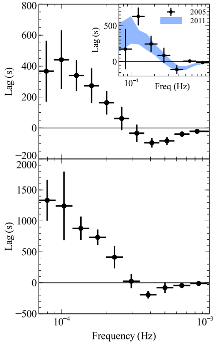
Figure 2. The lag as a function of temporal frequency for Ark 564. The lag is measured between 0.3–1 keV and 1.2–4 keV (top) and between 0.3–1 keV and 4–7.5 keV (bottom). The amplitudes of the soft and hard lags are much larger in the bottom panel. However, we note that the frequency of the soft lag is the same for both energy ranges. The inset shows the 0.3–1 to 1.2–4 keV lag using only the 100 ks observation from 2005 (black points) overlaid with the 1\sigma contours of the 2011 lag-frequency spectrum in blue. The 2005 soft lag is not significant, but is consistent with the new observations.
