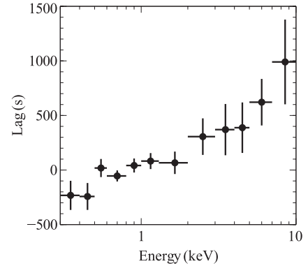
Figure 9. The low-frequency lag-energy spectrum of Mrk 335 in the low-frequency range [0.4\text{--}1.6] \times 10^{-4} Hz. Like Fig. 4 the profile appears smooth and very different from the high-frequency lag-energy spectra.
