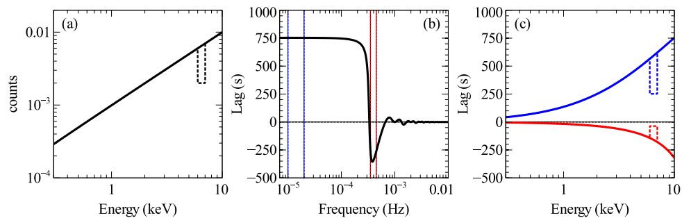
Figure 10. Model of the lag-energy spectra given a simple top-hat response function for two test cases: (1) where the reflection fraction increases steadily with energy (solid line) and (2) where the reflection fraction increases steadily with energy except for a demonstrative dip at 6 to 7 keV (dotted line). We show the reflection spectrum (a), the lag-frequency spectrum (b) and the low- and high-frequency lag-energy spectrum (c) shown in blue and red, respectively.
