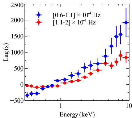
Figure 4. The low-frequency lag-energy spectrum of Ark 564 in the low-frequency range [0.6-1.1] \times 10^{-4} Hz (blue) and [1.1-2] \times 10^{-4} Hz (red). The profile is smooth and very different from the high-frequency lag-energy spectra.
