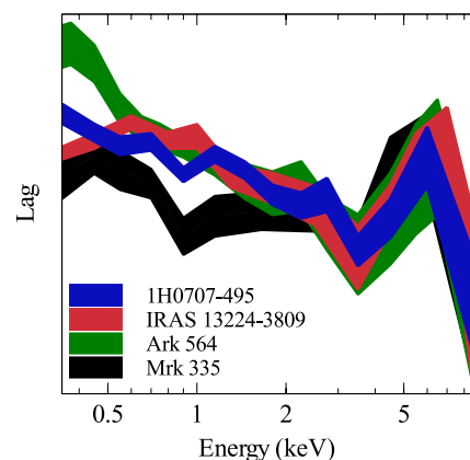
Figure 11. The high-frequency lag-energy profiles for four of the seven sources that exhibit Fe K lags, including 1H0707–495 (blue), IRAS 13224–3809 in at low fluxes (red), Ark 564 (green) and Mrk 335 (black). As the zero-point is arbitrary, the lags have been scaled to the 3 to 4 keV band. The Fe K lag profile is the same in all four sources, but the lags at the soft excess do not share a common shape.
