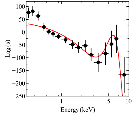
Figure 3. The lag-energy spectrum of Ark 564 in the frequency range [3.2\text{--}5.2] \times 10^{-4} Hz. The lag-energy profile shows a peak at the energy of the Fe K line, and is similar to the soft lag-energy profiles seen in 1H0707–495 and IRAS 13224–3809. The red line shows the best-fitting linear model with an additional Gaussian at 6.4 keV.
