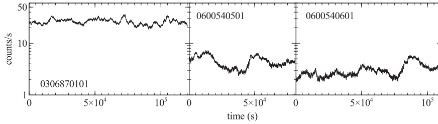
Figure 6. Mrk 335 broad-band light curve from 0.3–10 keV in 200 s bins. Note the logarithmic y-axis. The 2006 observation (left) is \sim 10 times brighter than the 2009 observations (middle, right).
