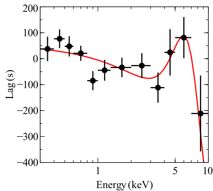
Figure 8. The Mrk 335 lag-energy spectrum in the frequency range [1.9\text{--}6.7] \times 10^{-4} Hz. Only the data from 2006 were used as no lag was present in the 2009 observation. The red line shows the best-fitting linear model plus a Gaussian at 6.4 keV.
