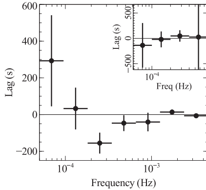
Figure 7. The Mrk 335 lag as a function of temporal frequency between 0.3–0.8 keV and 1–4 keV for the 2006 observations. The inset shows the lag as a function of frequency for just the 2009 low-flux observations. No lag was detected, and therefore we did not use these observations in the lag-energy analysis.
