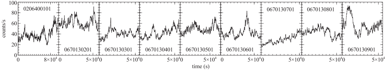
Figure 1. Ark 564 broad-band light curves from 0.3–10 keV in 200 s bins. For the purposes of comparing the counts rate between different observations, the light curves were all generated with circular source extraction regions with 35 arcsec radii. However, for the lag and spectral analysis, we accounted for pile-up by extracting annuli where needed. Note that the earlier observation (obsid 0206400101; leftmost panel) is longer, and is shown with a different x -axis scaling.
