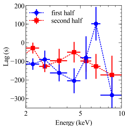
Figure 5. The lag-energy spectra of Ark 564 for the first half of the observation (obsid 201–501; blue) and the second half (obsid 601–901; red). The first half lag-energy spectrum is shown at \nu = [3.4-4.5] \times 10^{-4} Hz and the second half is shown at a slightly larger frequency range, \nu = [3.2-5.2] \times 10^{-4} Hz. The first half at lower frequencies clearly shows a narrower peak at 6 to 7 keV, while the second half at higher frequencies shows a broader feature peaking at 4 to 5 keV.
