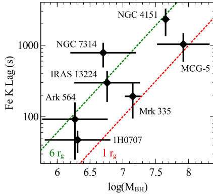
Figure 12. The amplitude of the Fe K lag versus M_{\text{BH}} for the seven Seyferts with detected Fe K reverberation lags. See Table 2 for details about the sources. The light crossing times at 1 r_g and 6 r_g as a function of mass are shown as red and green lines, respectively.
