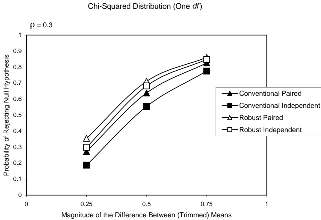
Figure 2. Probability of rejecting H_0 for the conventional and robust paired and independent-samples t tests; \rho = 0.3 .
