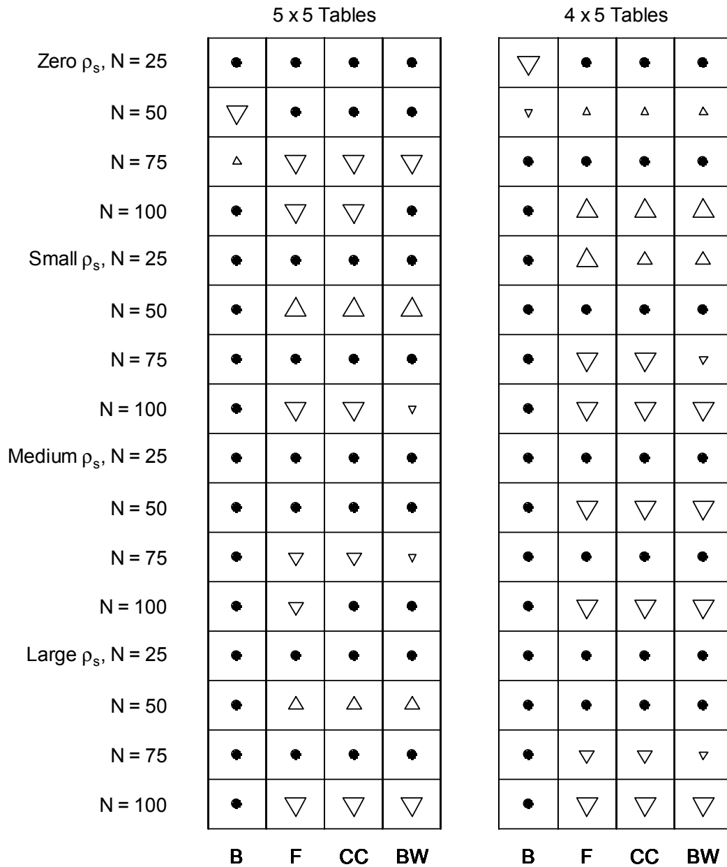
Figure 6: Chart indicates whether coverage was within the control limits of .95. These limits are [.9365, .9635] for \alpha = .05 , [.9322, .9678] for \alpha = .01 , and [.9273, .9727] for \alpha = .001 . B = bootstrap. F = Fieller, et al. (1957). CC = Caruso and Cliff (1997). BW = Bonnett and Wright (2000).
