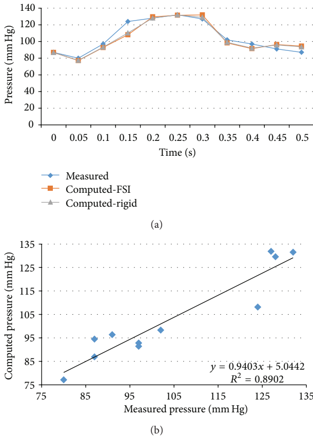
FIGURE 6: (a) depicts the pressure waveforms for the examined cardiac cycles (measured and computed results) and (b) exhibits the linear regression analysis for patient #2.
