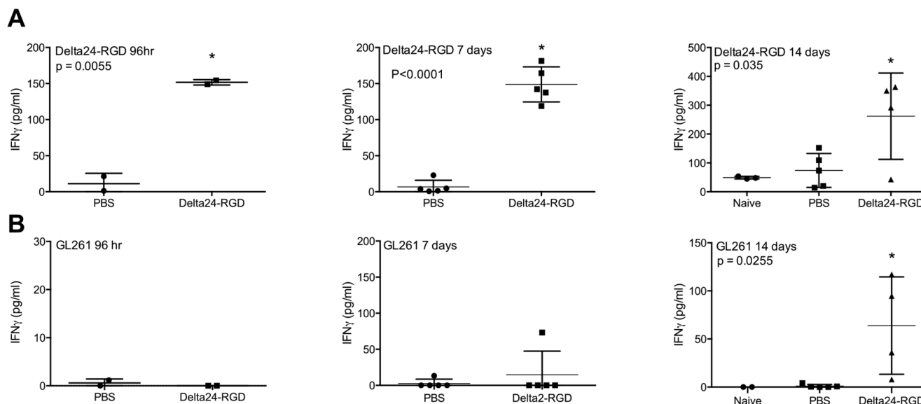
Figure 7. Delta24-RGD treatment of GL261 glioma induces virus and tumor specific T cells. IFN \gamma levels (in pg/ml \pm SD) in supernatants of splenocytes derived at 96 hr and 7 and 14 days after treatment from naïve, PBS and Delta24-RGD treated mice and cocultured with Delta24-RGD (A) or GL261 cells (B). The IFN \gamma levels were corrected for those produced by splenocytes cocultured with the control cell line A549. doi:10.1371/journal.pone.0097495.g007
