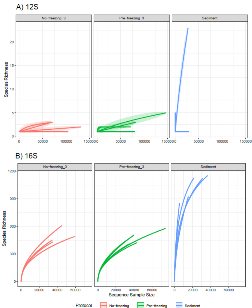
Figure 4 – Species rarefaction curves based on sequencing effort for each protocol. A) 12S primer; B) 16S primer. With the exception of the water samples for the 12S primer, none of the curves have reached a plateau, although we expect the high diversity seen for the 12S sediment samples be due to contamination from tag-jumping.
