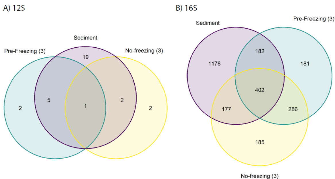
Figure 3 – Venn diagrams of A) 12S and B) 16S primers showing the number of species found at and between each protocol. Sediment samples showed the highest number of unique species for both primers, although for the 12S dataset, about 28% are the result of contamination from tag-jumping.
