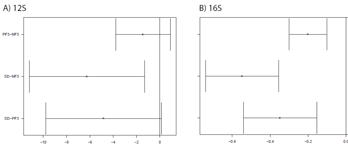
Figure 5 – Confidence interval (CI) for slopes of rarefaction curves (Fig. 3) for each pairwise comparison of the different protocols. Only the comparison between pre- versus no freezing water samples, and pre-freezing versus sediment samples for the 12S primer (A) have come out non significant. The remaining comparisons showed significant differences between rarefaction slopes.
