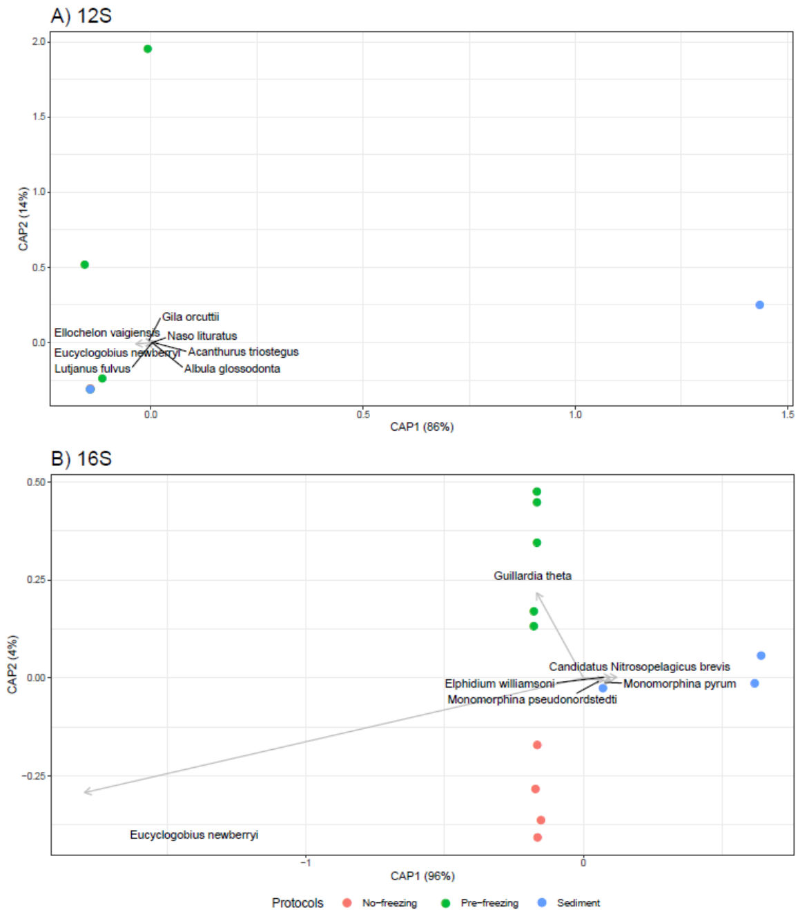
Figure 9 – Constrained Analysis of Principal Coordinates (CAP) of rarefied A) 12S and B) 16S primer datasets. Circles are colored by protocol. While there were no discernible differences in assemblage composition for the 12S primer, in the 16S primer Guillardia theta is overrepresented in the PF protocol in comparison to the NF protocol. Eucyclogobius newberryi is underrepresented in the sediments compared to the filtration protocols, especially the NF protocol.
