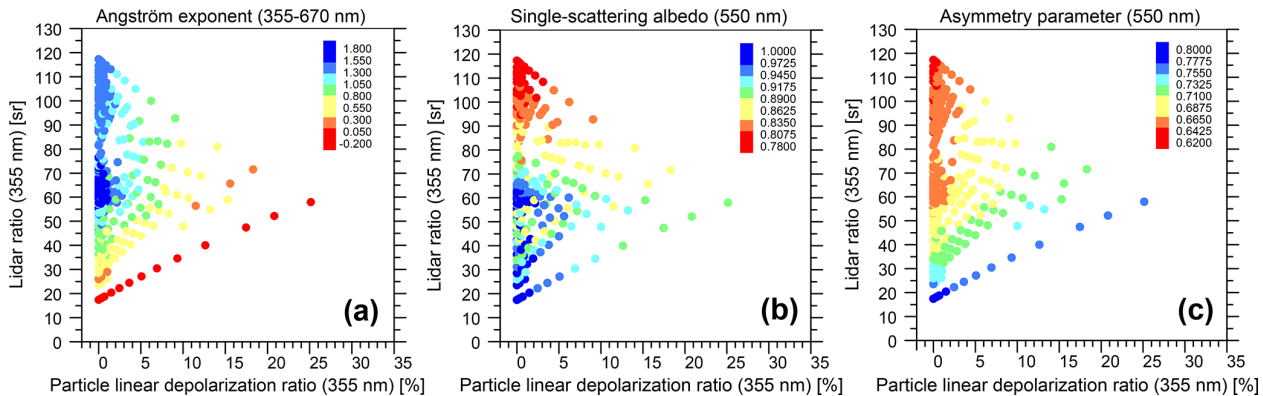
Figure 8. Simulated values of (a) Ångström exponent for the 355–670 nm spectral range, (b) single-scattering albedo at 550 nm, and (c) asymmetry parameter at 550 nm. The values are color coded and projected into the S – \delta plane at 355 nm (see legends).
