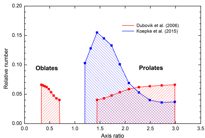
Figure 3. Axis ratio distribution proposed by Dubovik et al. (2006), shown in red, and by Koepke et al. (2015), shown in blue. The latter one is interpolated from the original linear to the logarithmic grid needed for calculations with Dubovik's code for spheroid scatterers. The logarithmic grid is indicated by the symbols.
