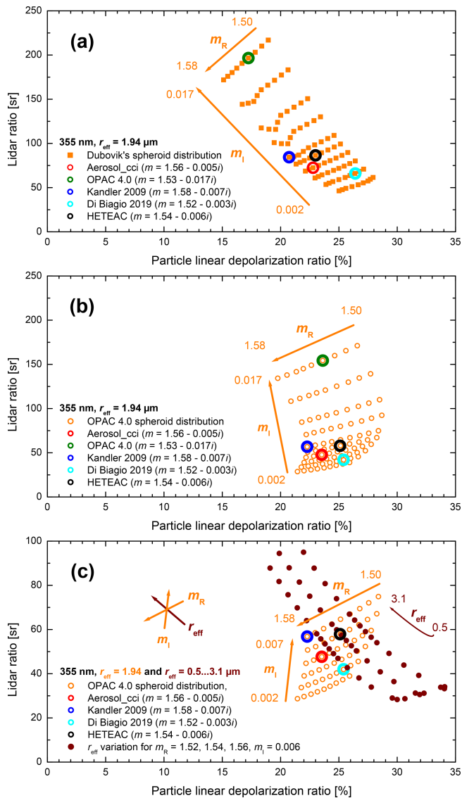
Figure 5. Simulated values of lidar ratio versus particle linear depolarization ratio at 355 nm for (a) the spheroid distribution after Dubovik et al. (2006) and (b, c) the spheroid distribution after Koepke et al. (2015). Orange symbols show results for a constant effective radius of 1.94 \mu\text{m} and a varying complex refractive index as indicated in the figure. Dark-brown symbols in panel (c) show results for a varying effective radius.
