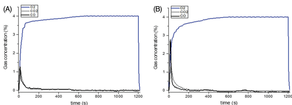
Figure 9. Concentration profile of the 5 th oxidation cycle in the FBR cycling experiment at 850°C using 15 vol% CO + N 2 for the reduction and 4 vol% O 2 + N 2 for the oxidation: (A) Fe 2 O 3 -MM sample and (B) Fe 2 O 3 -CP sample. The gas flow rate was kept constant to maintain a value of u/u_{mf} of 3.
