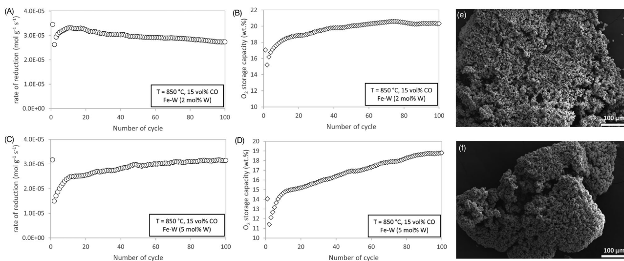
Figure 8. The maximum observed rate of reduction and Ro measured in the TGA at 850 °C over 100 redox cycles using 15 vol% CO + N 2 for the reduction and 4 vol% O 2 for the oxidation: (A) observed rate and (B) Ro for the FeW-2-CP oxygen carrier and (C) observed rate and (D) Ro for the FeW-5-CP oxygen carrier, and SEM images of an oxygen carrier particle recovered after 100 redox cycles of the (E) FeW-2-CP and (F) FeW-5-CP, SE micrographs with (E, F) ×200 magnification.
